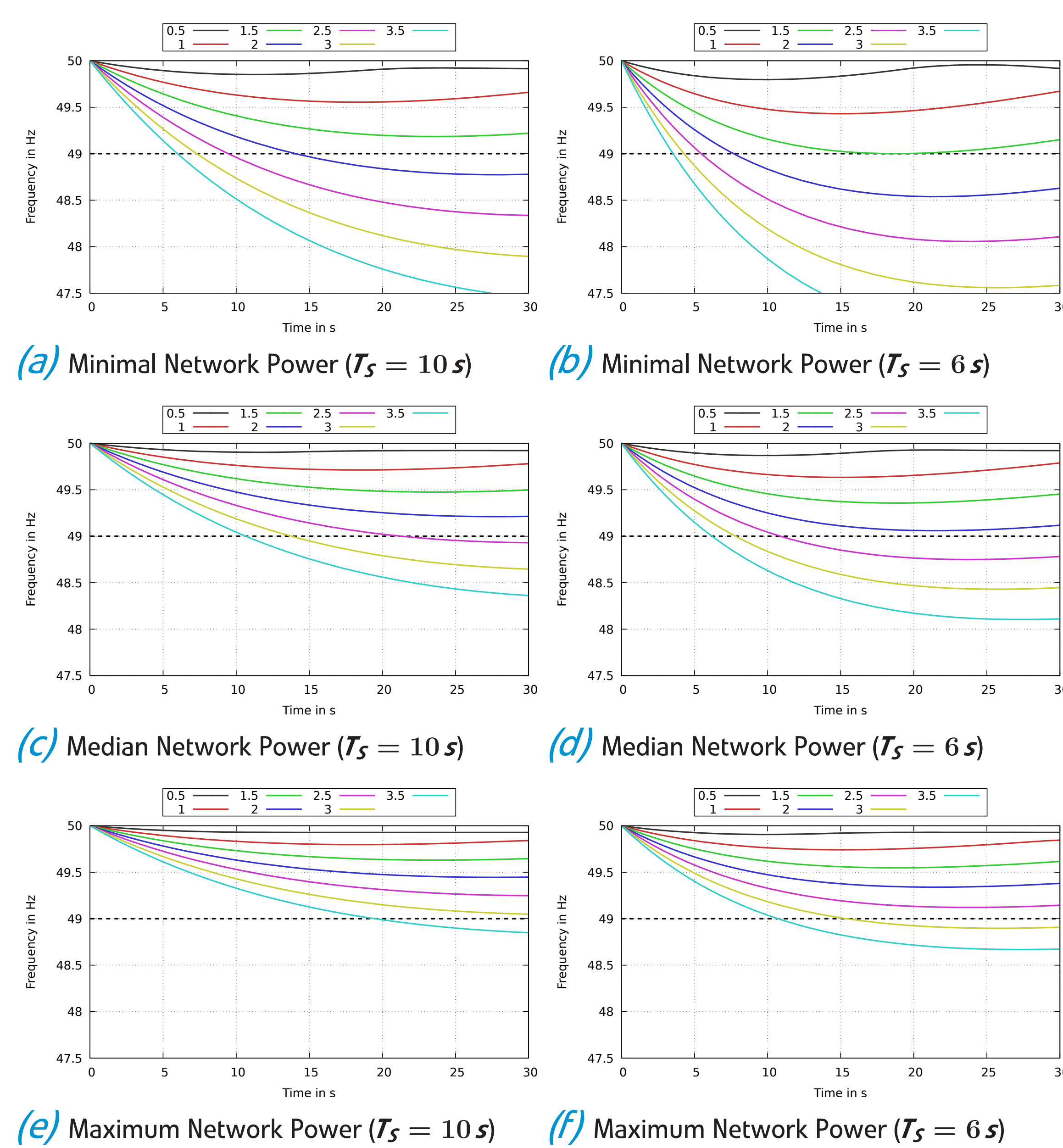
Figure 1: Impact of Static Load Attacks on Grid Frequency
